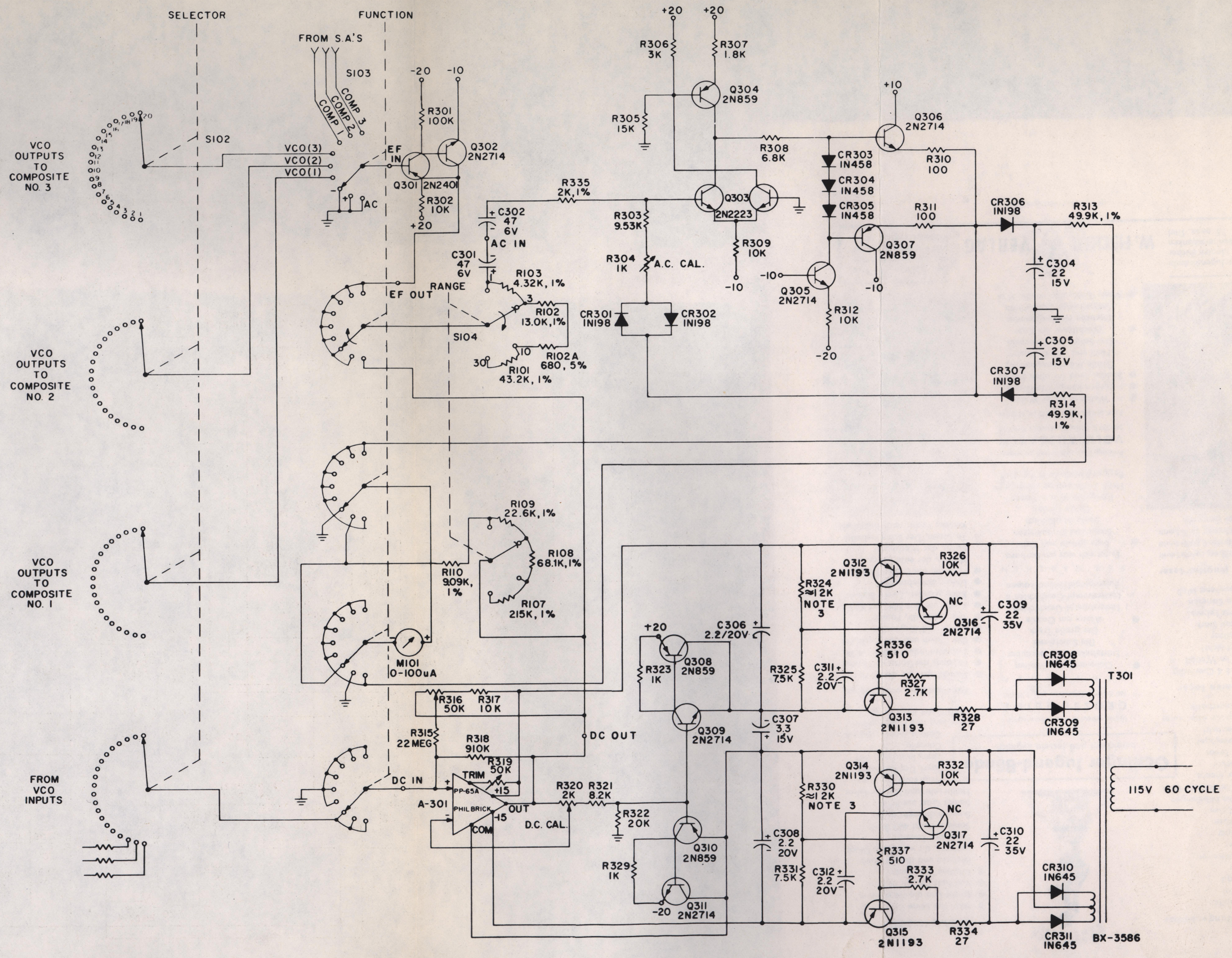
Figure 7-3. Model DIC-1A Meter Circuit, Schematic Diagram R30-838
