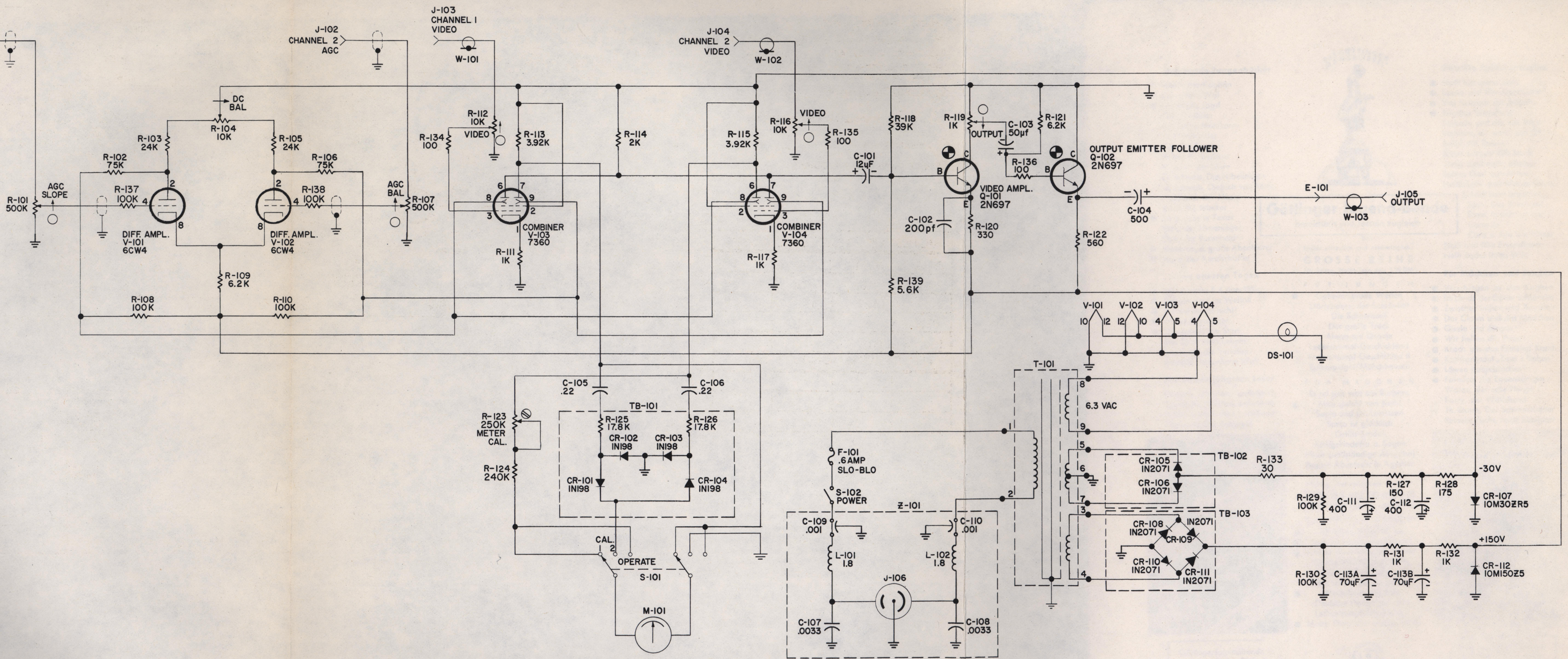
Figure 6-1. Model TDC-1B Diversity Combiner Schematic Diagram R13-811
